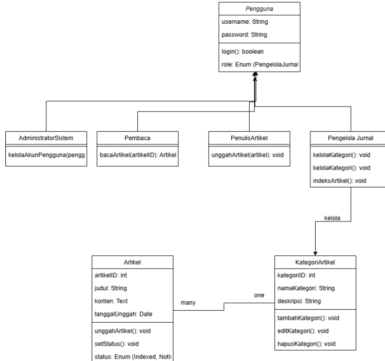
Gambar 10. Class Diagram
