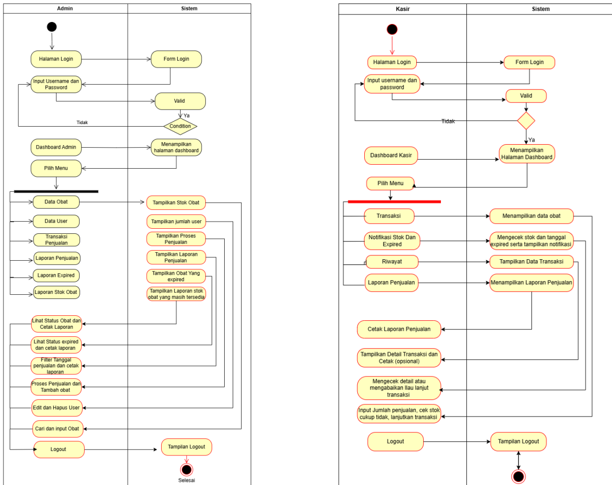
Gambar 3. Activity Diagram Admin dan Activity Diagram Kasir
