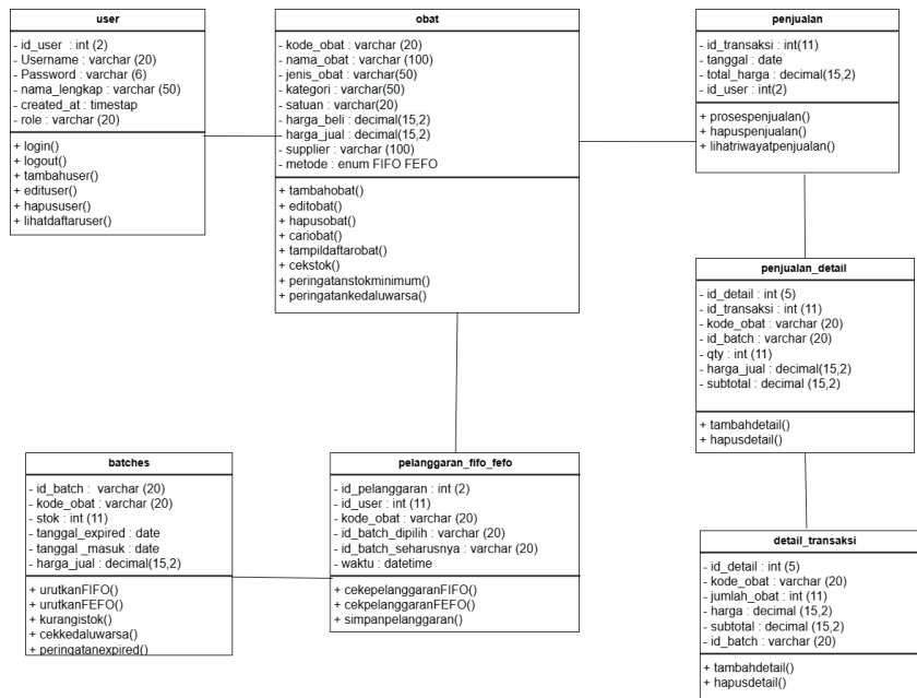
Gambar 4. Class Diagram Rancangan Tabel Relasi
