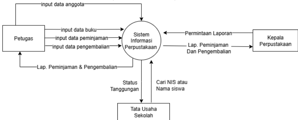
Gambar 2. DFD (Data Flow Diagram)
