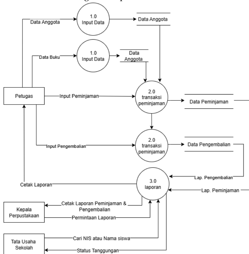
Gambar 3. DFD Level 1
